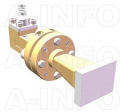
LB-12-15-C-1.0FSPO Standard Gain Horn Antenna 60-90GHz 15dB Gain 1.0mm Female
